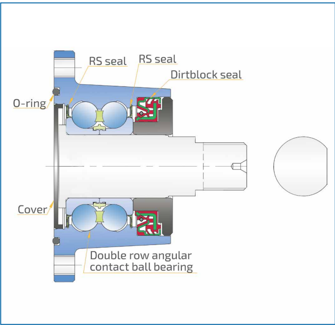
Fig.14. Technical drawing of Agro Point Hub IL50
